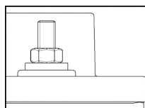
Screw-Terminal + M6-Bold-Adapter
