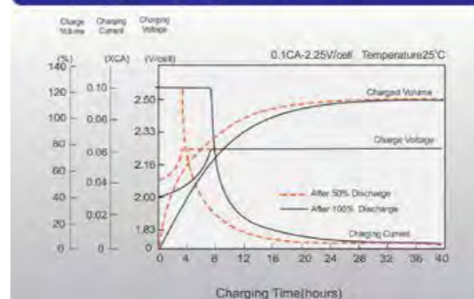
Floating Charging Characteristics
