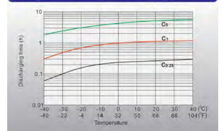
Temperature Effect on Discharging Time
